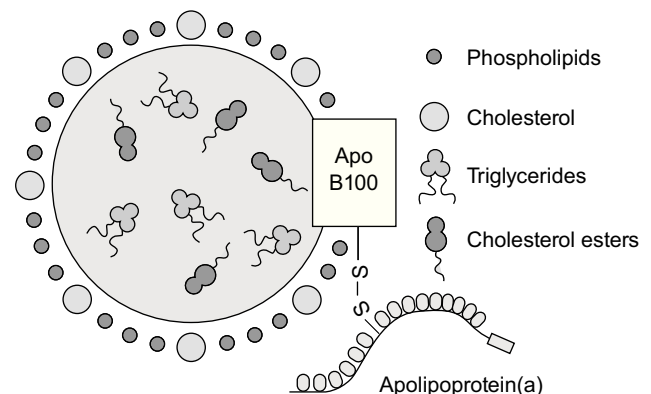
Figure 1 Structure of lipoprotein (a).
